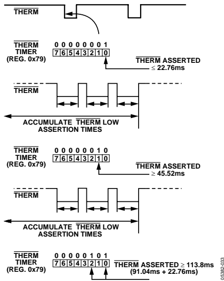
Figure 32. Understanding the \overline{THERM} Timer
