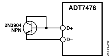
Figure 26. Measuring Temperature Using an NPN Transistor
