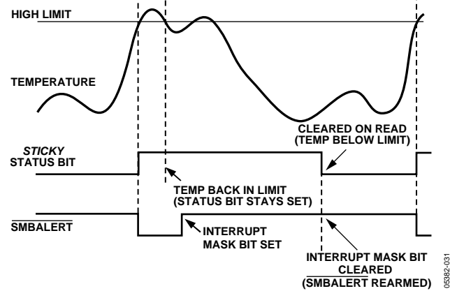
Figure 30. How Masking the Interrupt Source Affects SMBALERT Output
