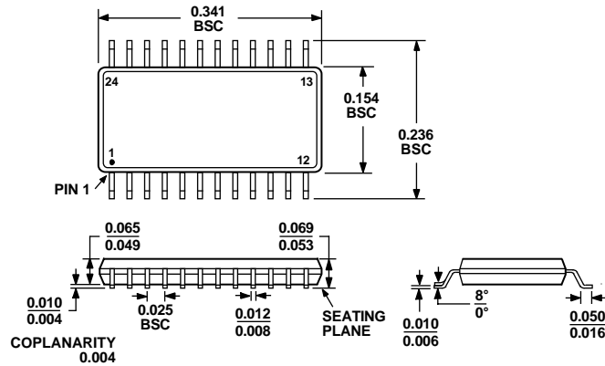
Figure 67. 24-Lead Shrink Small Outline Package [QSOP] (RQ-24)
