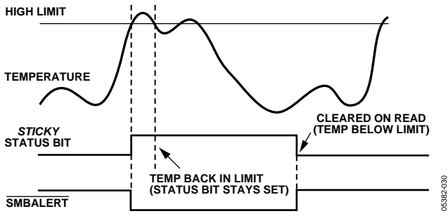
Figure 29. SMBALERT and Status Bit Behavior
