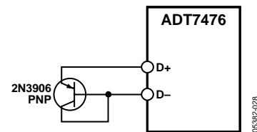
Figure 27. Measuring Temperature Using a PNP Transistor
